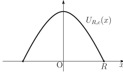
Figure 5.1: The graph of U_{R,c}(x) .
