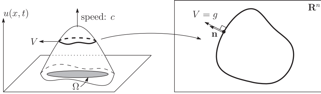
Figure 1.1: Growth laws in the case of (5).
