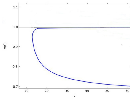
Figure 1.1: In blue, the branch of radially nondecreasing solutions u of (1), plotted as u(0) as function of q . Both the upper and the lower parts of such a branch seem to persist for all values of q . Moreover, the blue branch do not bifurcate from the one of constant solutions u \equiv 1 . The figure is obtained numerically with the software AUTO-07p [13], for problem (1) with p = 1.97 in dimension N = 1 .
