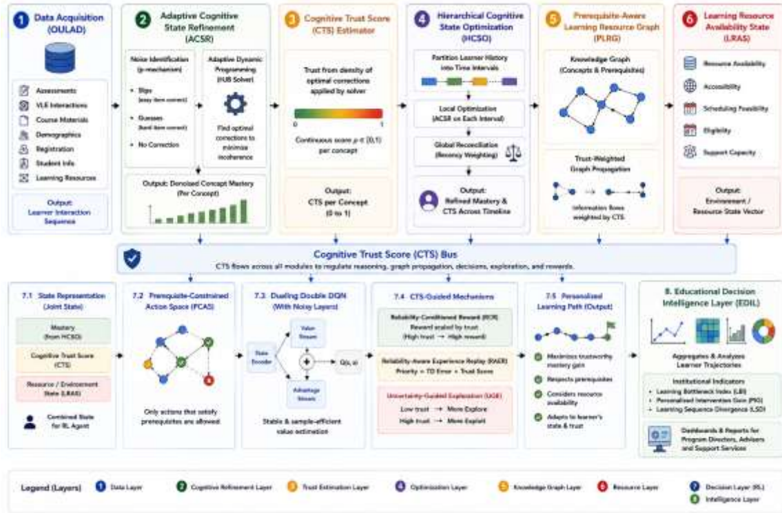
Figure 1 Proposed CTPLF architecture. The eight numbered stages group into the four modules described in Section 3: stages 2 to 4 form ACSR with HCSO, stage 5 the PLRG, stage 7 the CTGLPN, and stage 8 the EDIL.
