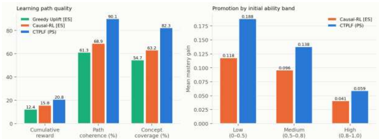
Figure 3 Learning path quality and knowledge state promotion by initial ability band
