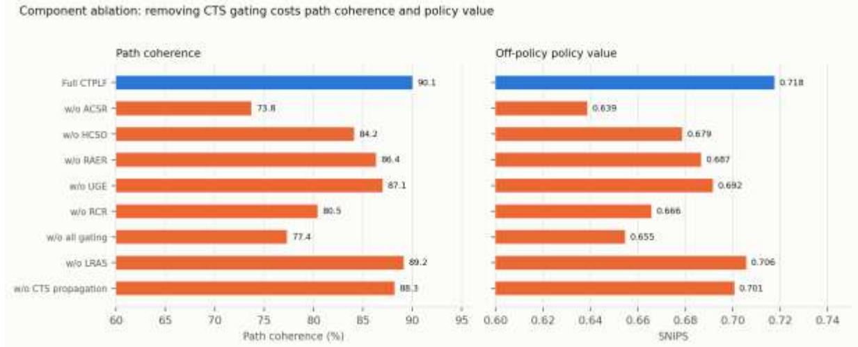
Figure 7 Component ablation across path coherence and off-policy policy value
