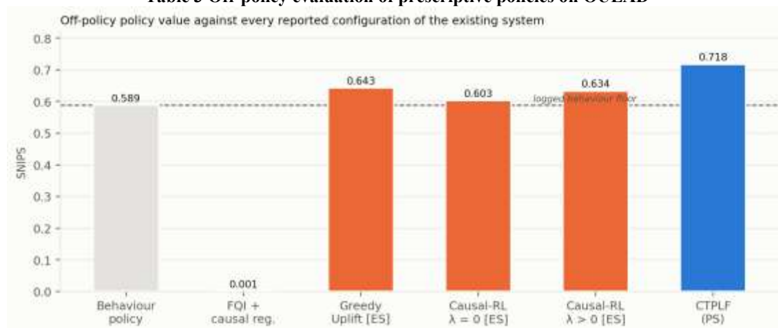
Figure 2 Off-policy policy value against every reported configuration of the existing system
