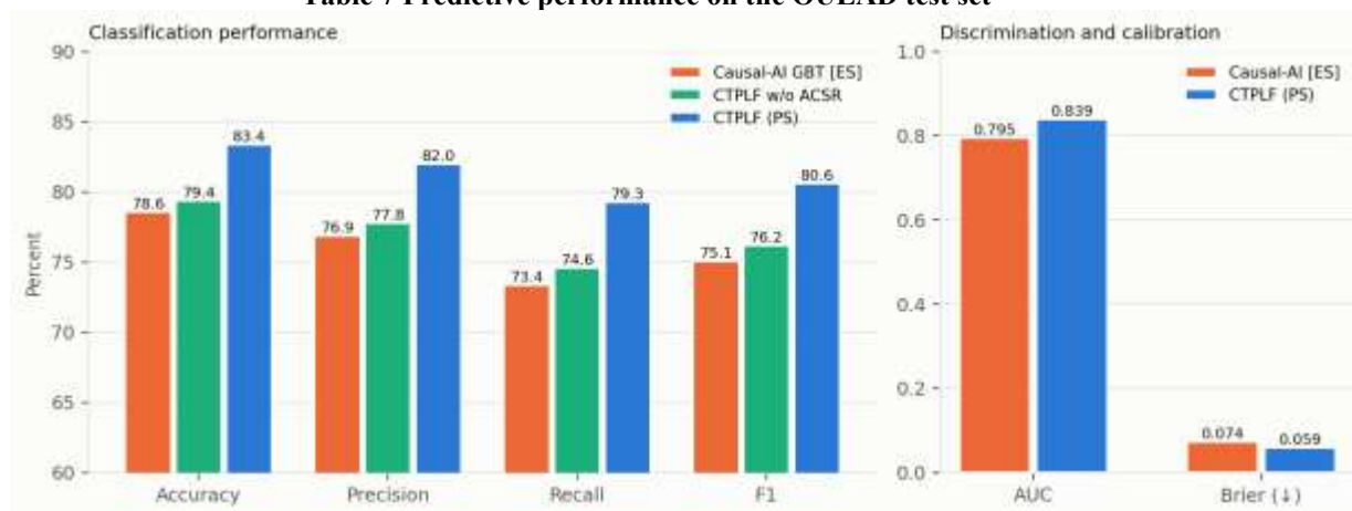
Figure 4 Predictive validation against the existing system on OULAD
