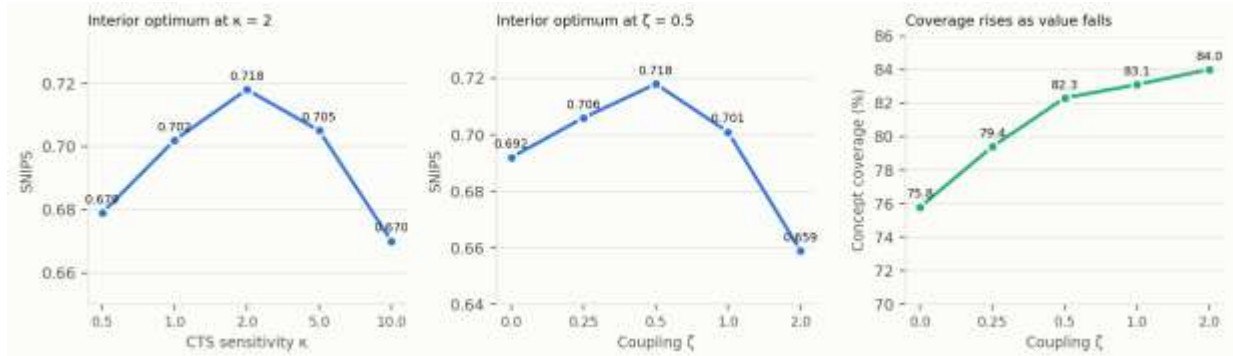
Figure 8 Sensitivity of framework performance to the CTS coefficients \kappa and \zeta
