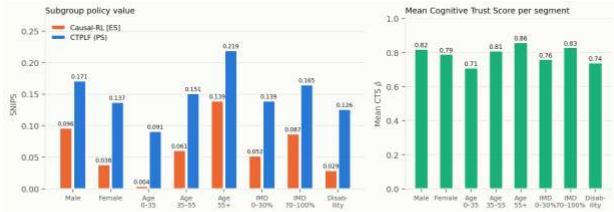
Figure 5 Subgroup policy value and mean Cognitive Trust Score across OULAD segments
