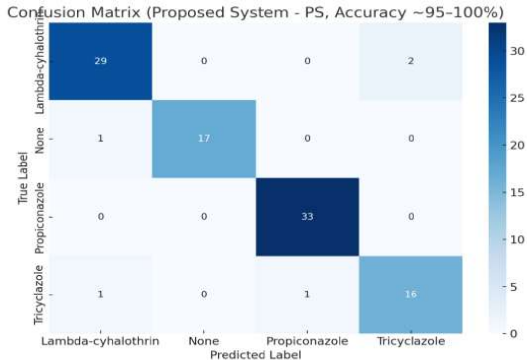
Figure 6. Confusion matrix of the proposed system
