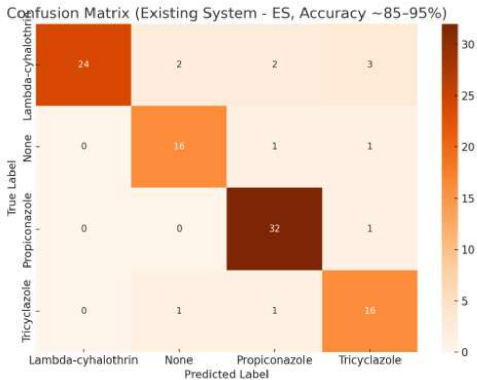
Figure 5. Confusion matrix of existing system
